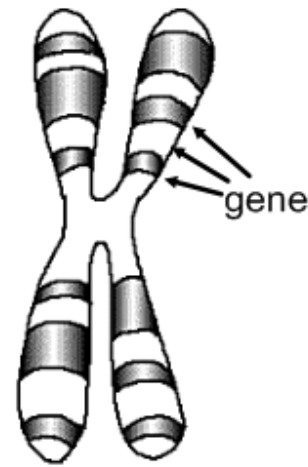
Chromosome
